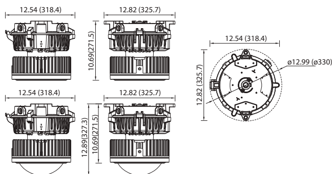
Pendant/Ceiling
