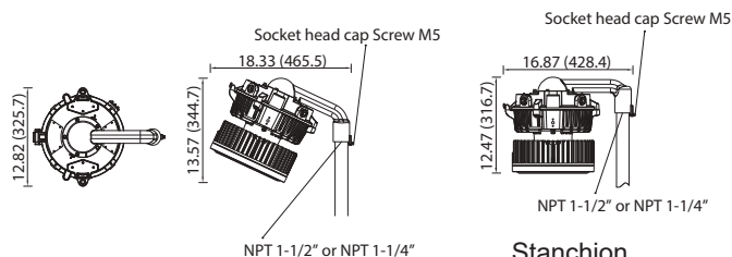
Stanchion
