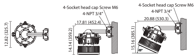
Wall
