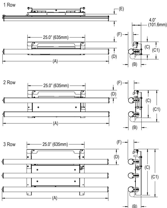
MOUNTING BRIDGE DETAIL (P/N: 18518)
