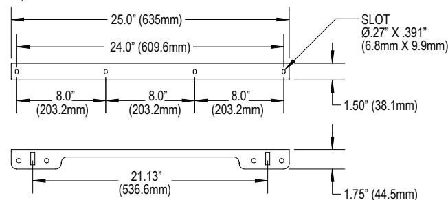
MOUNTING BRIDGE DETAIL (P/N: 18518)
