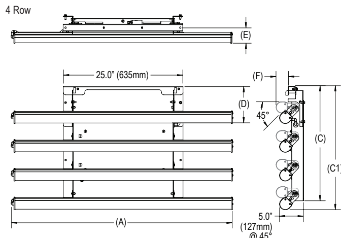
MOUNTING BRIDGE DETAIL (P/N: 18518)
