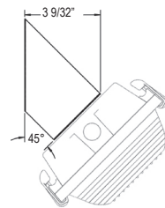
45° Mounting option
