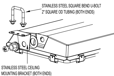
Ceiling mount system kit 8367 - Square bend U bolt
