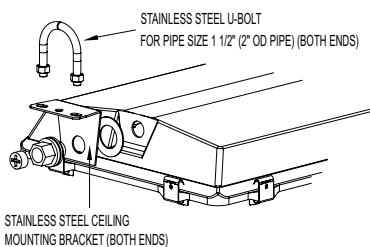
Ceiling mount system kit 8368 - U bolt
