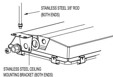
Ceiling mount system kit 8369 - 3 Ft. rod
