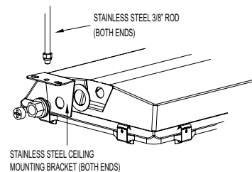
Ceiling mount system kit 8369 - 3 Ft. rod
