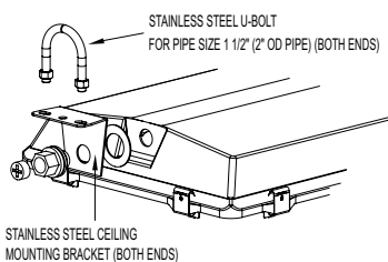
STAINLESS STEEL CEILING MOUNTING BRACKET (BOTH ENDS)
