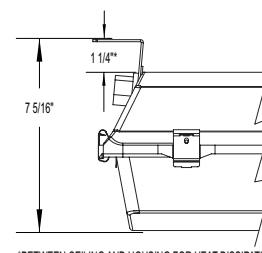
Ceiling mount system kit 8369 - 3 Ft. rod
