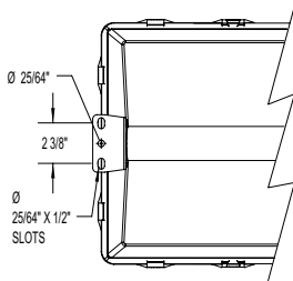
Ceiling mount system kit 8367 - Square bend U bolt
