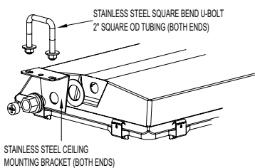
STAINLESS STEEL CEILING MOUNTING BRACKET (BOTH ENDS)
